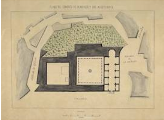
Floor plan of the convent of La Merced and its surroundings (1901)
