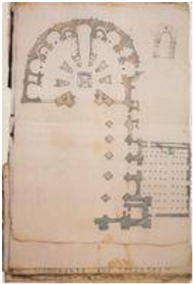
Floor plan of the Granada cathedral and the church of El Sagrario (1594). Juan de la Vega
